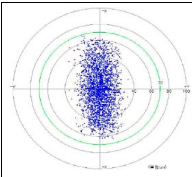
Figure 10. 'Skewed' X-axis hole scatter.
