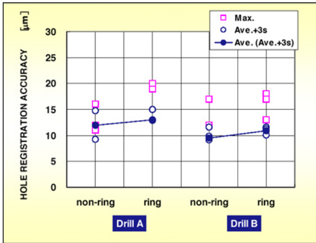
Figure 12. The influence of drill shank-rings on hole registration.
