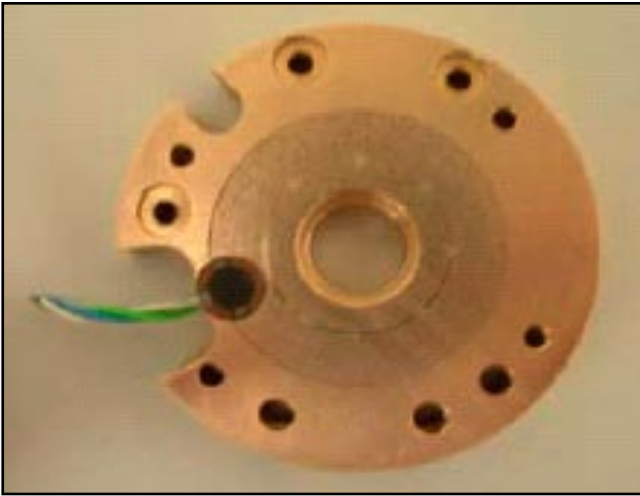
Figure 3. View of axial bearing plate.
