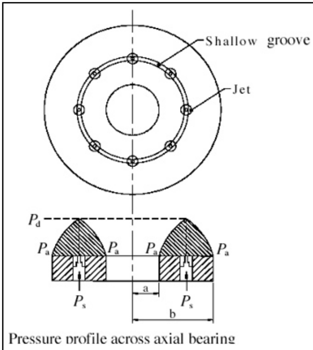
Figure 4. Axial/thrust geometry in aerostatic bearing.
