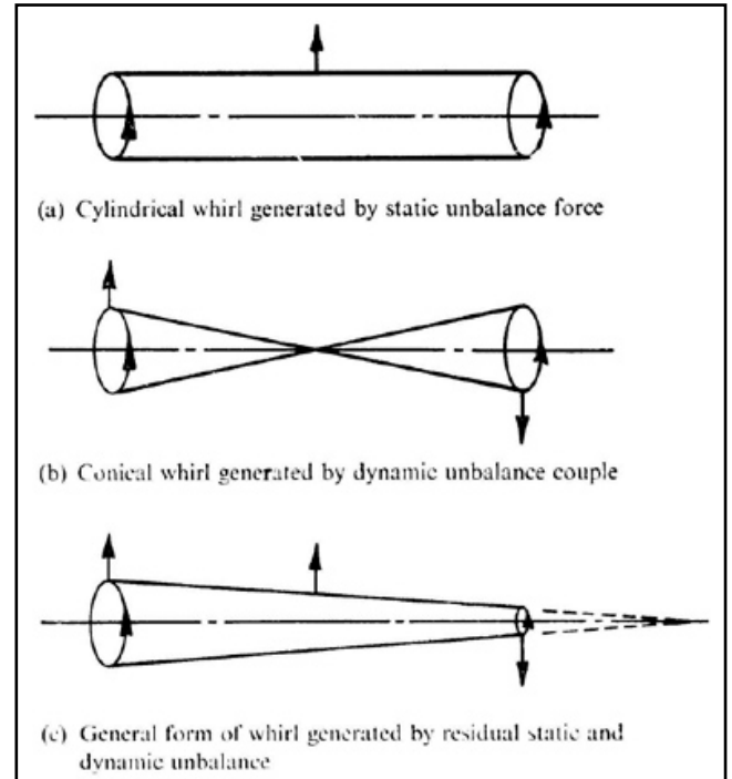
Figure 6. Effects of residual unbalance on shaft motion.
