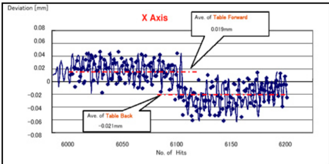
Figure 9. Magnitude of deviations due to X-axis positioning.
