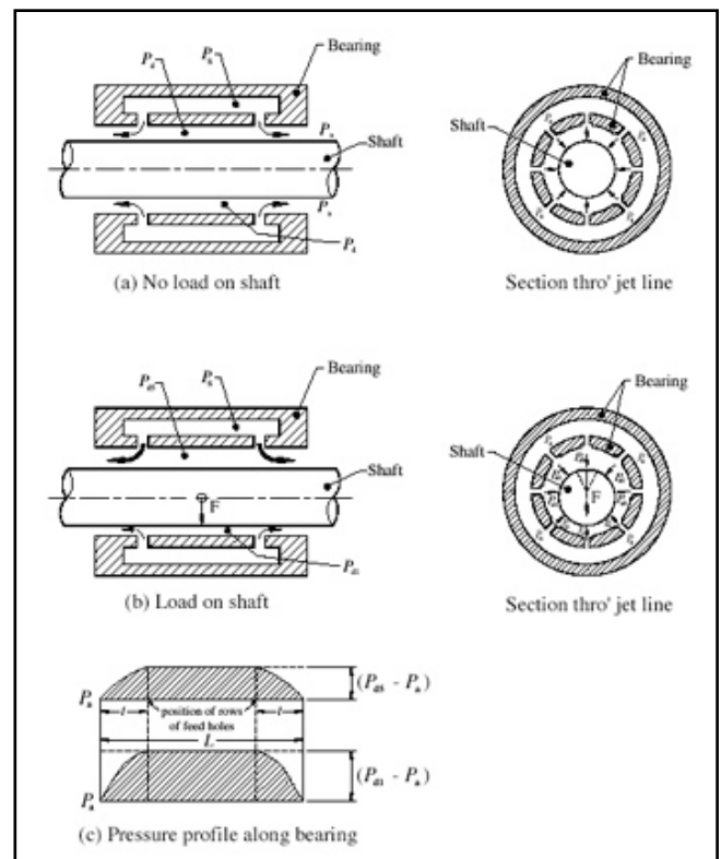
Figure 2. Radial geometry in aerostatic bearing.
